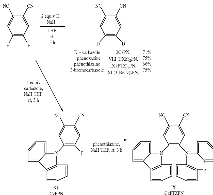
Scheme 2: synthesis of VIII, IX, X, intermediate XII and 3-bromocarbazole variant XI
